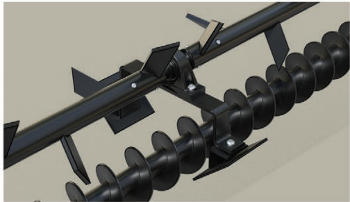
Steel auger (bottom) and anti-bridge bar (top) ensure clog-free asphalt conveyance and consistent heating.
