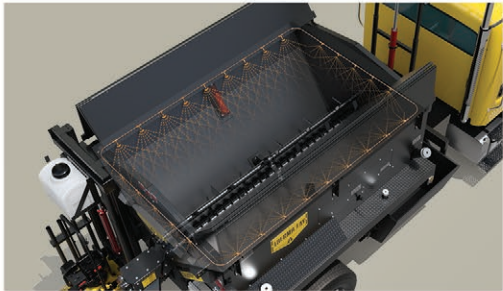
Release agent spray bar coats hopper to prevent asphalt from sticking, so crews don't have to climb truck or enter hopper.
